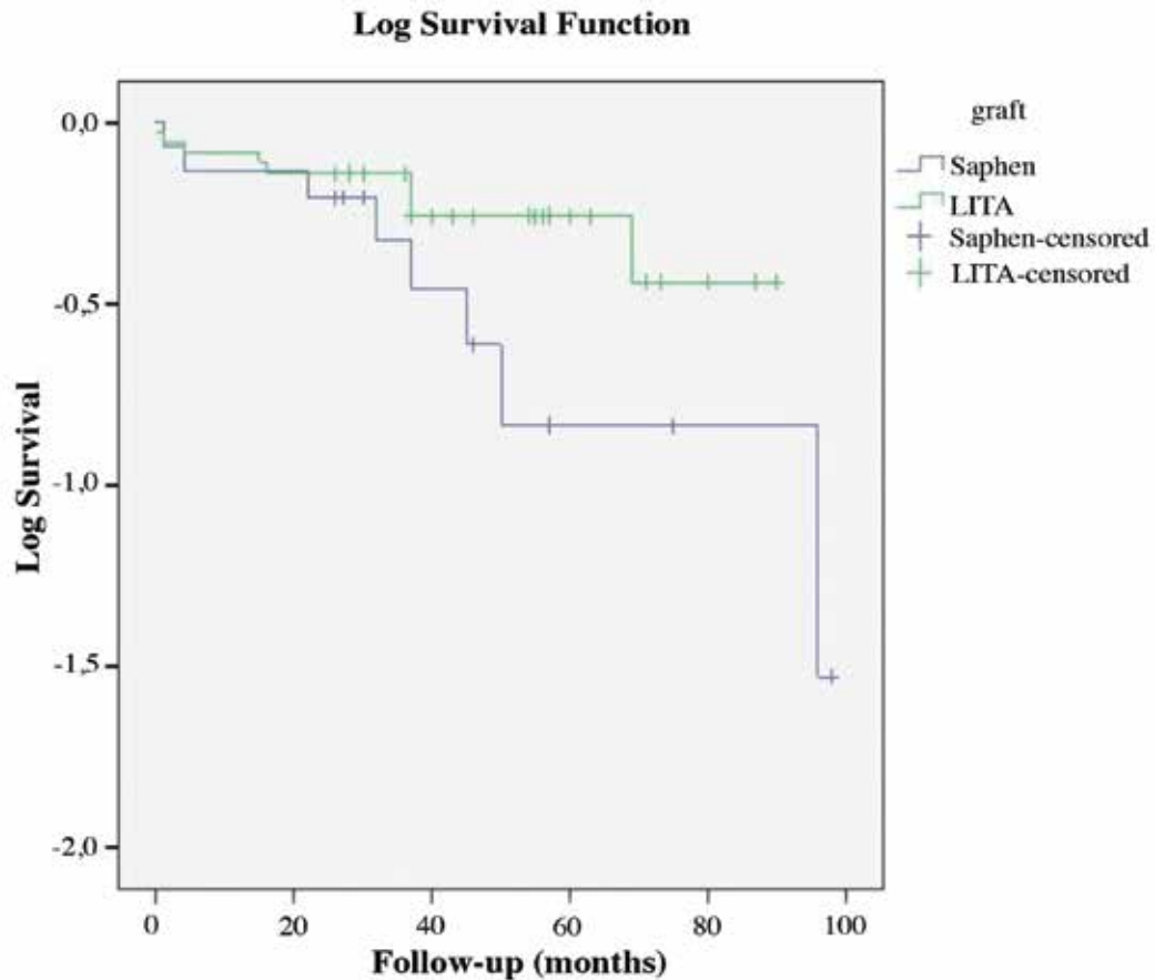
Figure 1. Survival graph.
